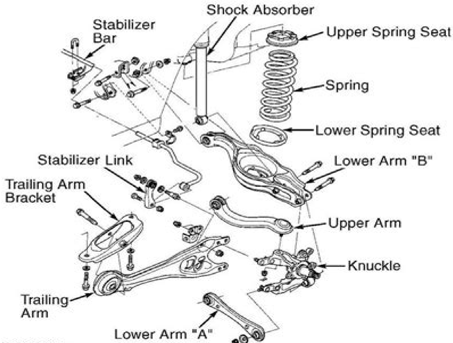
Fig. 5: Exploded View Of Rear Suspension (Odyssey) Courtesy of AMERICAN HONDA MOTOR CO., INC.
