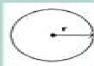
Circumference of a Circle and Area of a Circular Region
