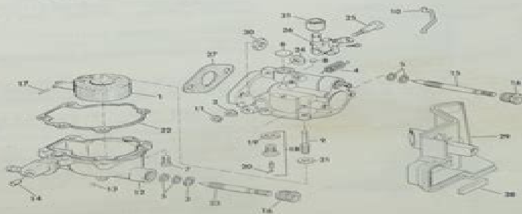
Carburetor Assembly (Exploded)
