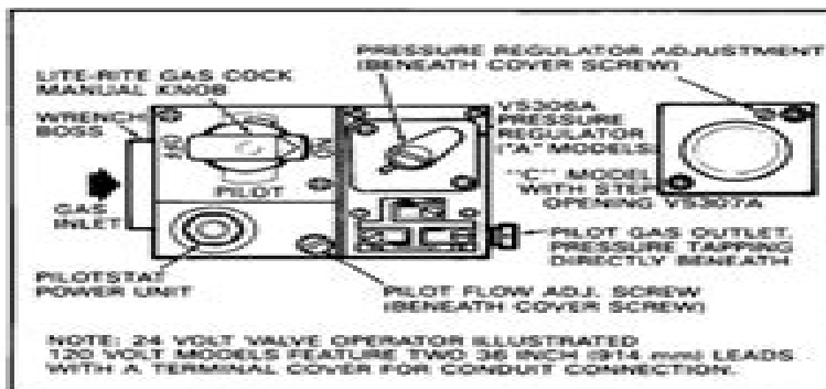
Fig. 1 — Top view A model. Pressure regulator for "C" model illustrated at right. (Blank cover plate (Part No. 392782) is available to convert an "A" model to a "B" model without pressure regulator.)
