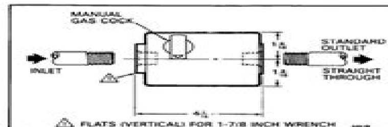
Fig. 2 — Piping pattern and dimensions (in inches) of VS820.
