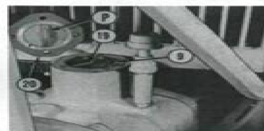
Fig. C506 — Manual steering gear for general purpose and high clearance models. Upper spindle end play is adjusted with plug (19). "O" ring (9) must be in good condition.
