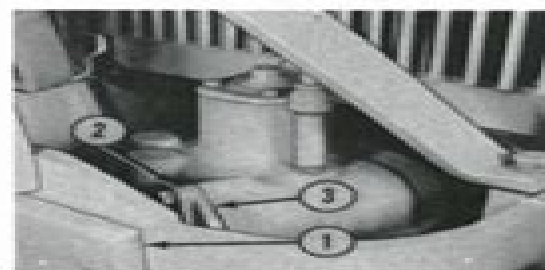
Fig. C505—Manual steering gear installation on general purpose and high clearance tractors. Steering worm shaft end play is adjusted with shims (3) between gear housing and front bearing carrier (2).
