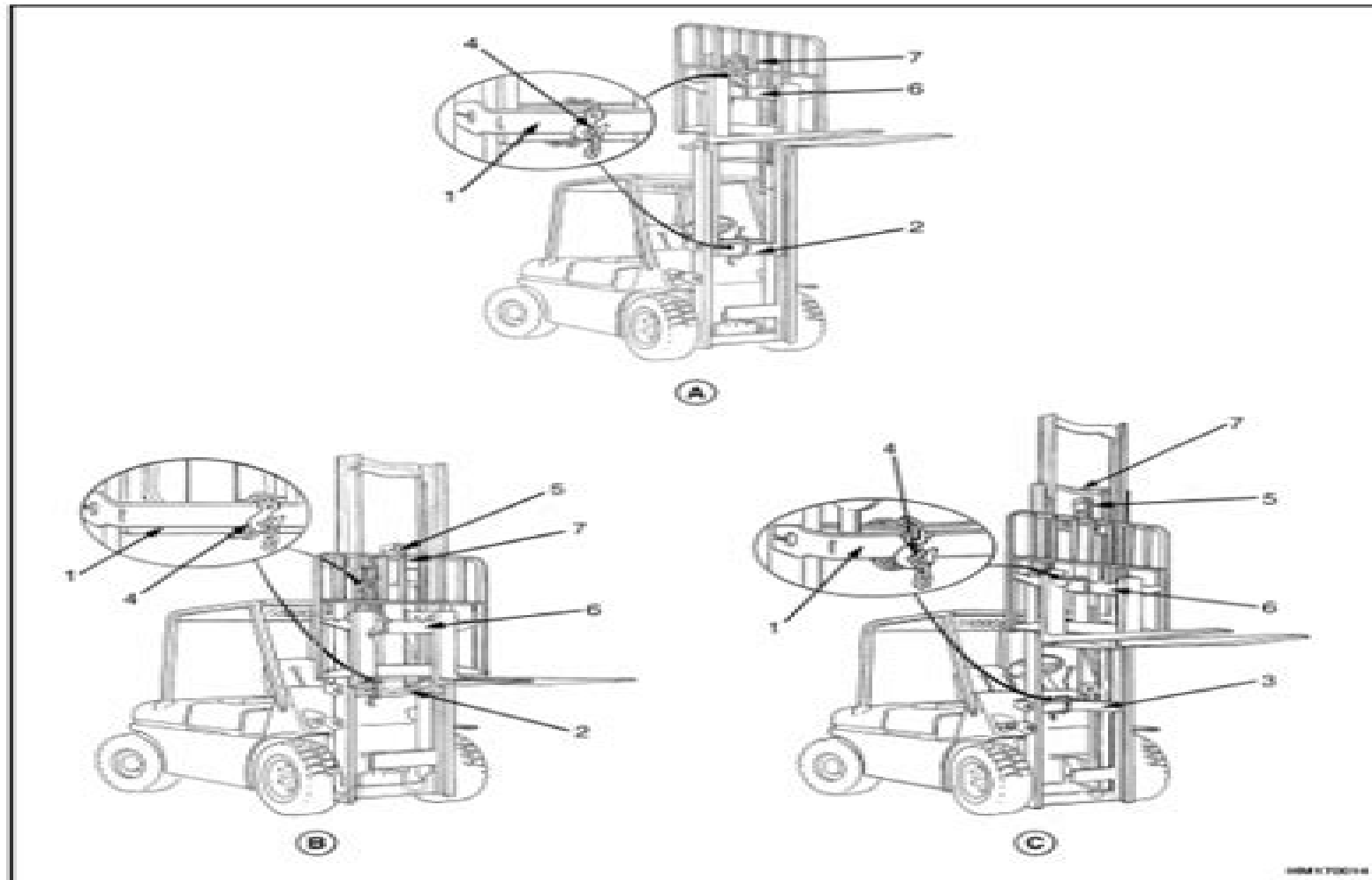
A. TWO-STAGE LFL MAST
