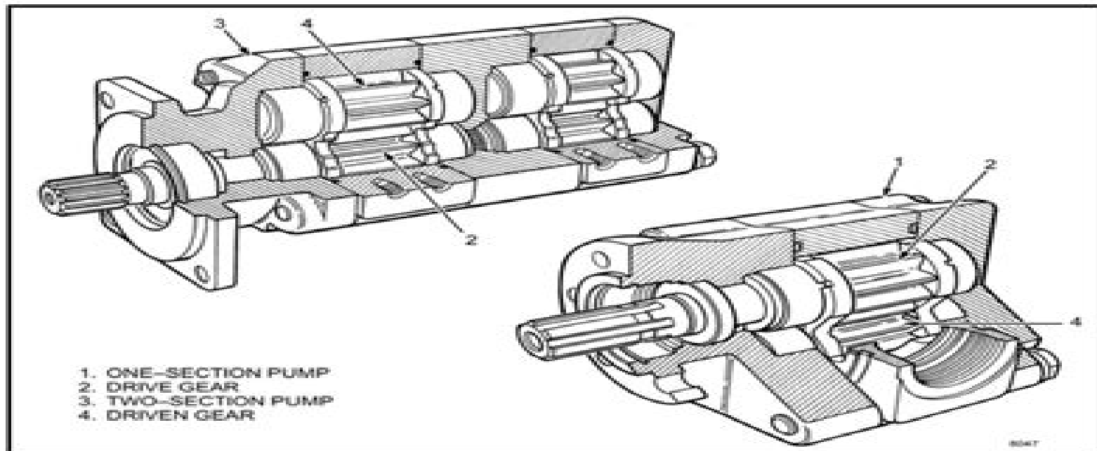
FIGURE 1. TYPES OF GEAR PUMPS
