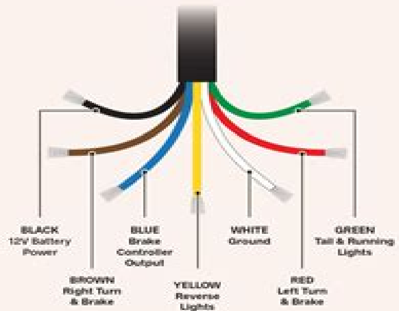
Wiring Side
