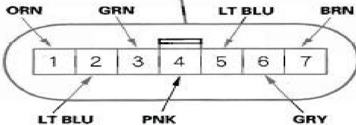
Wire side of female terminals
