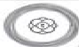
Nucleus with electrons that have calculated probable areas where they are located, but no exact location can be determined
