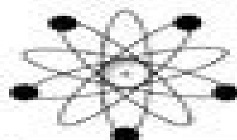
positively charged center with orbiting negatively charged particles
