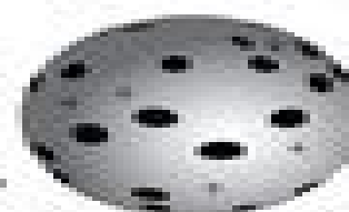
positively charged, low density, spacious body
