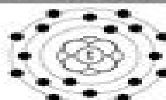
Nucleus with protons, neutrons, and electrons must orbit at defined energy levels and electrons away from the nucleus
