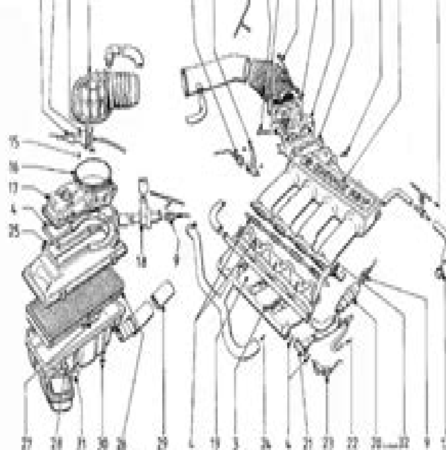
Fig. 4. Jetronic system (line manifold) and associated components - file engine
