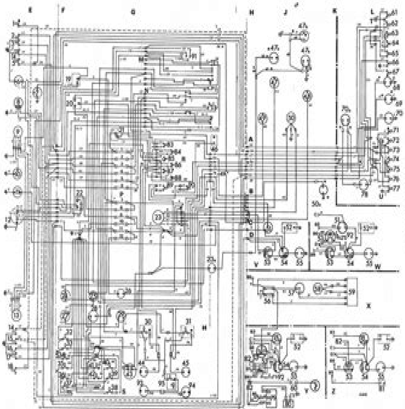
WIRING DIAGRAM
