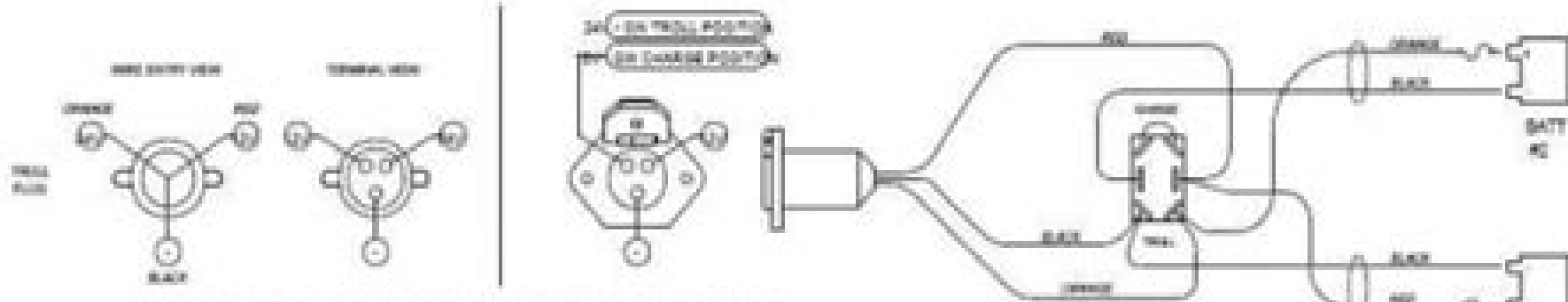
12/24 VDC 4-WIRE SWITCHED TROLLING / CHARGING WIRE SET
