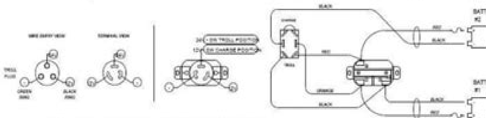
12/24 VDC 4-WIRE SWITCHED TROLLING / CHARGING WIRE SET
