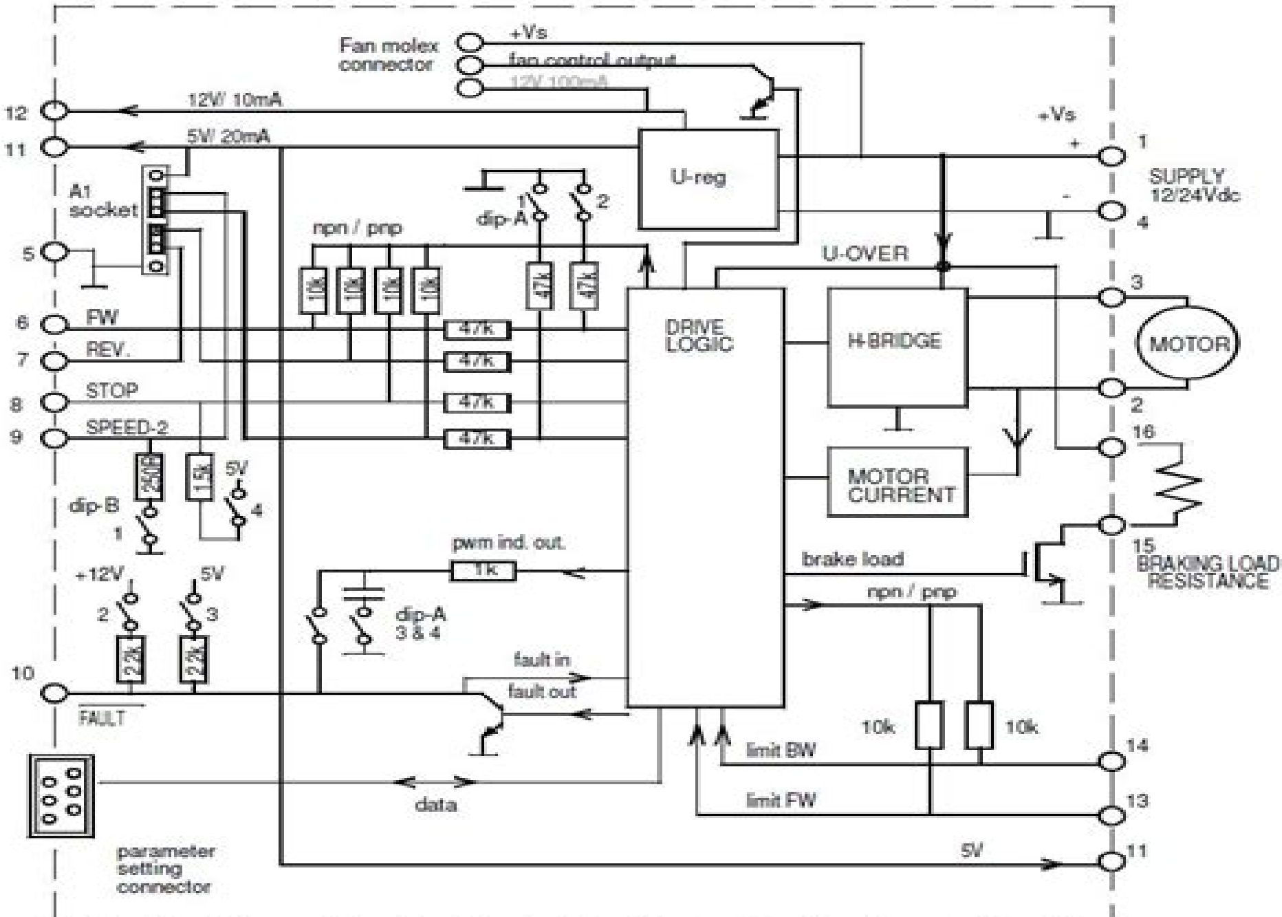
EM-362 BLOCK DIAGRAM
