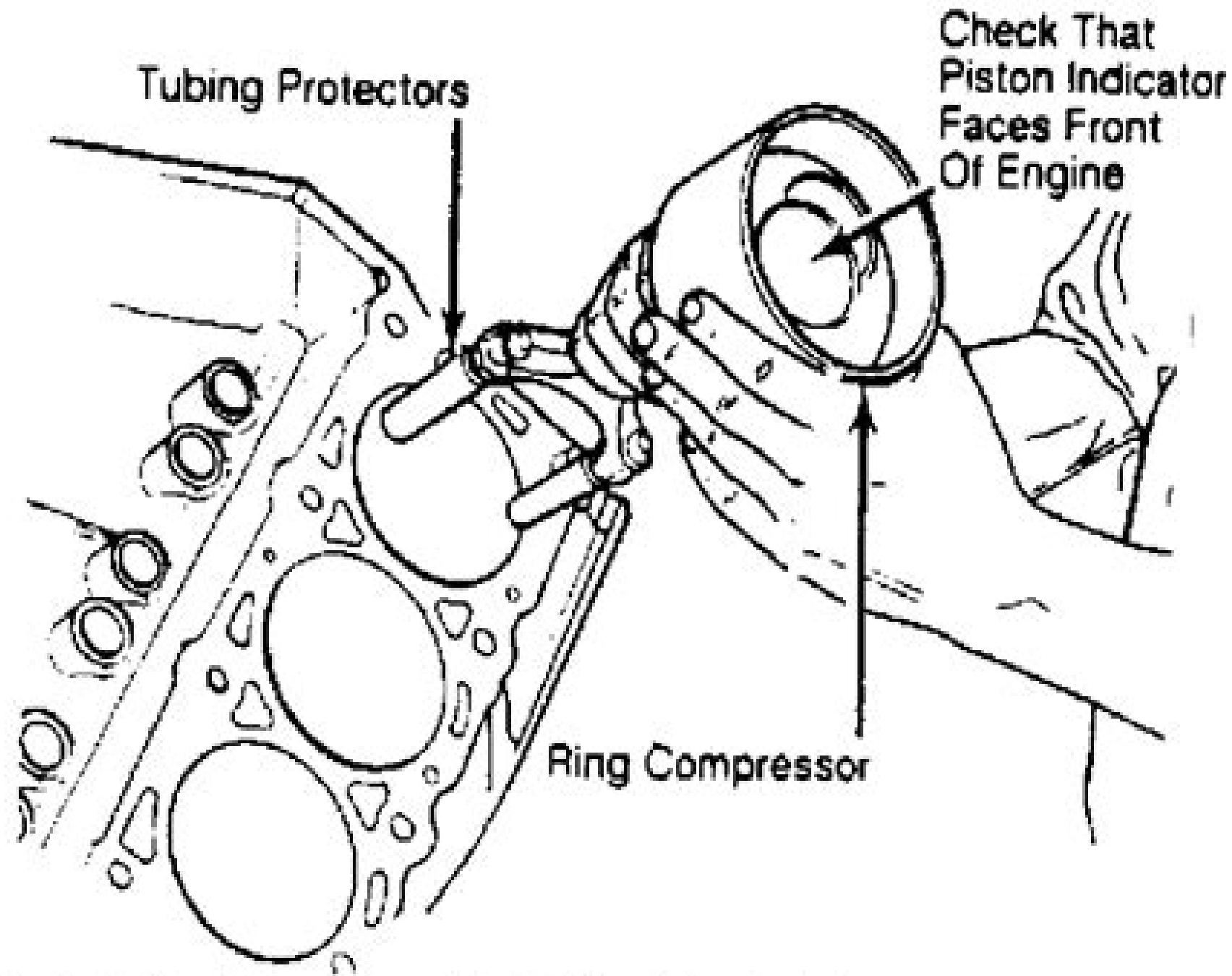
Fig. 17: Installing Piston & Connecting Rod Assembly - Typical This Graphic For General Information Only
