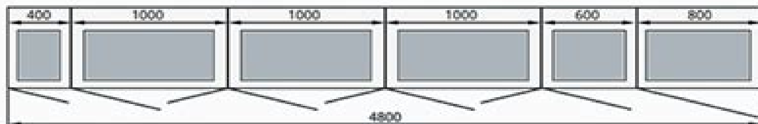
Installation front
