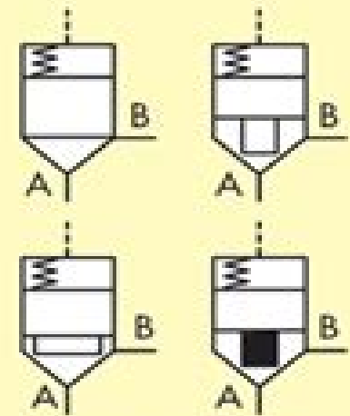
Logic Operators
