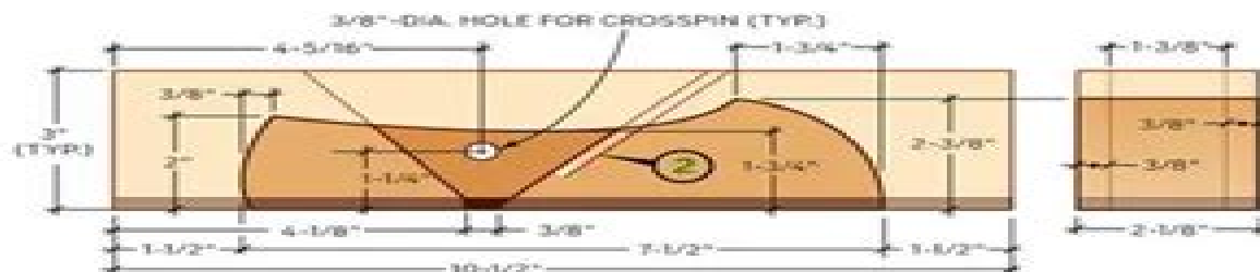
A — BLOCK PLANE SECTION VIEW
