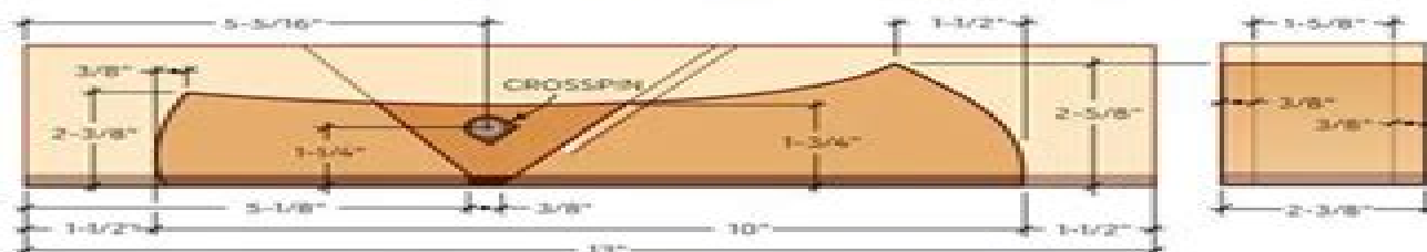
B — SMOOTH PLANE SECTION VIEW
