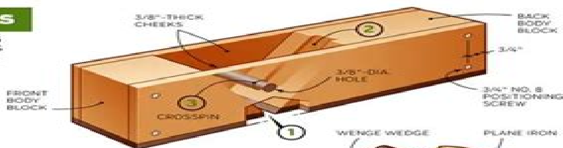
ASSEMBLED PLANE BLANK
