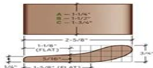
DETAIL 4 — WEDGE
