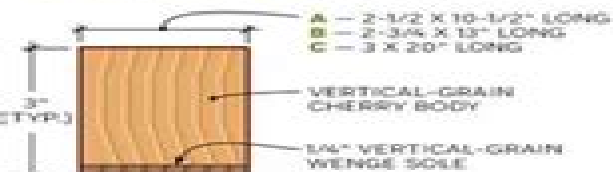
ROUGH BLANK
