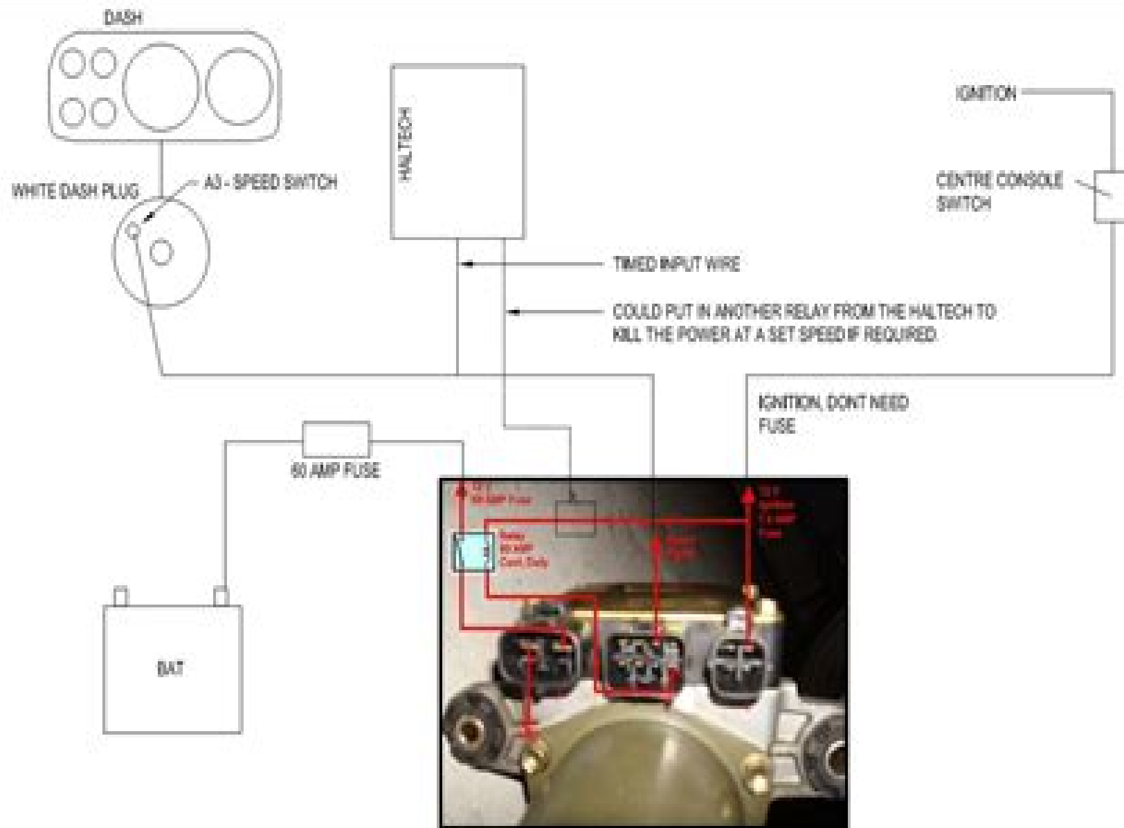
Anth's FC3S EHPS WIRING SETUP
