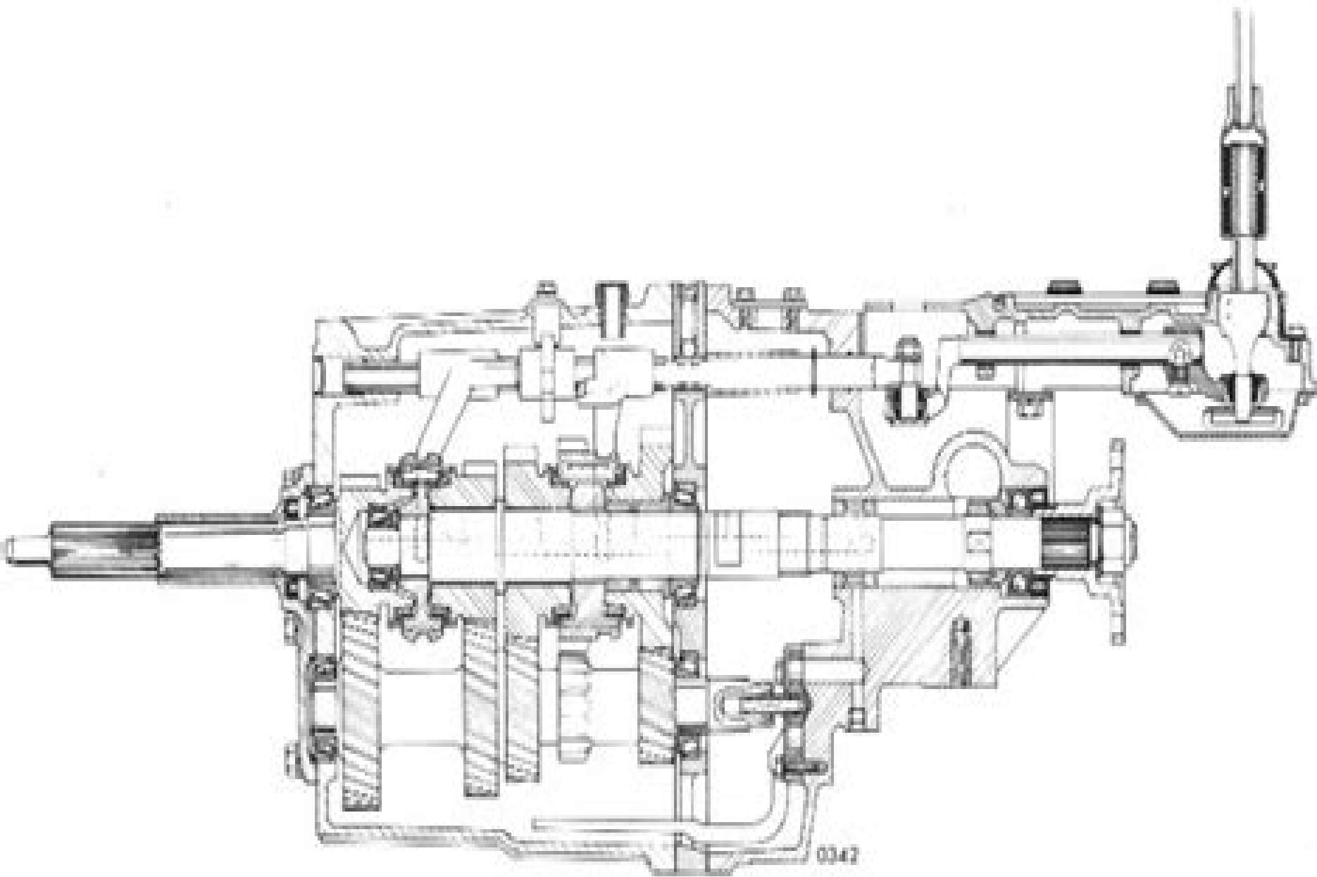
GEARBOX - 4-SPEED
