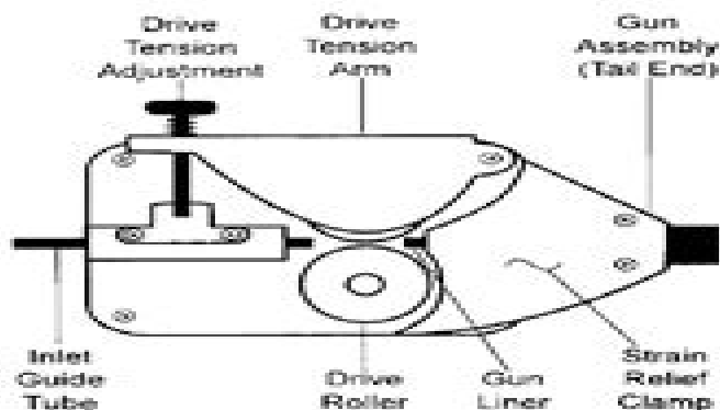
Figure 18. Drive Assembly
