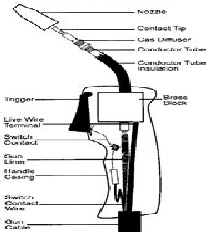
Figure 19. Gun Assembly
