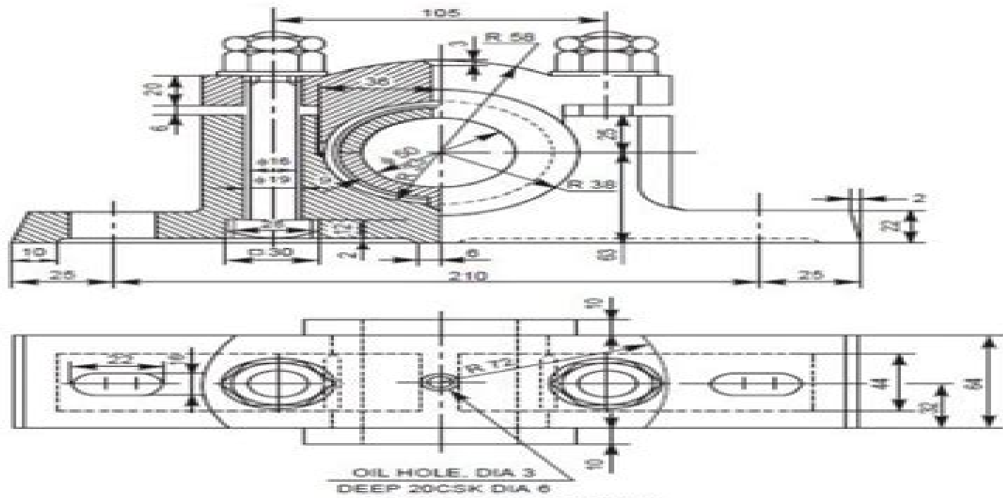
Fig. 12.4 Plummer block
