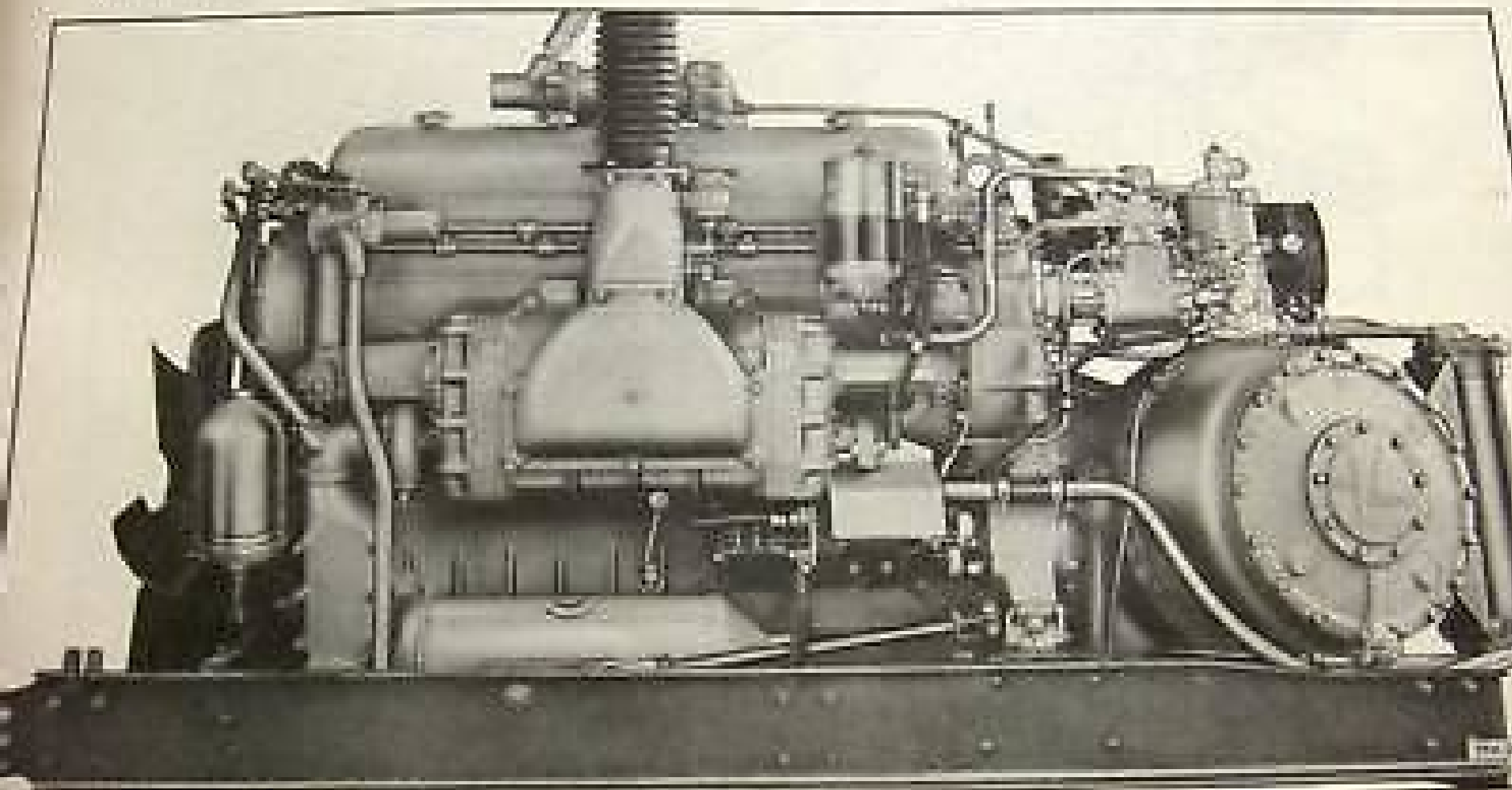
Figure 1—Transit Coach Power Plant
