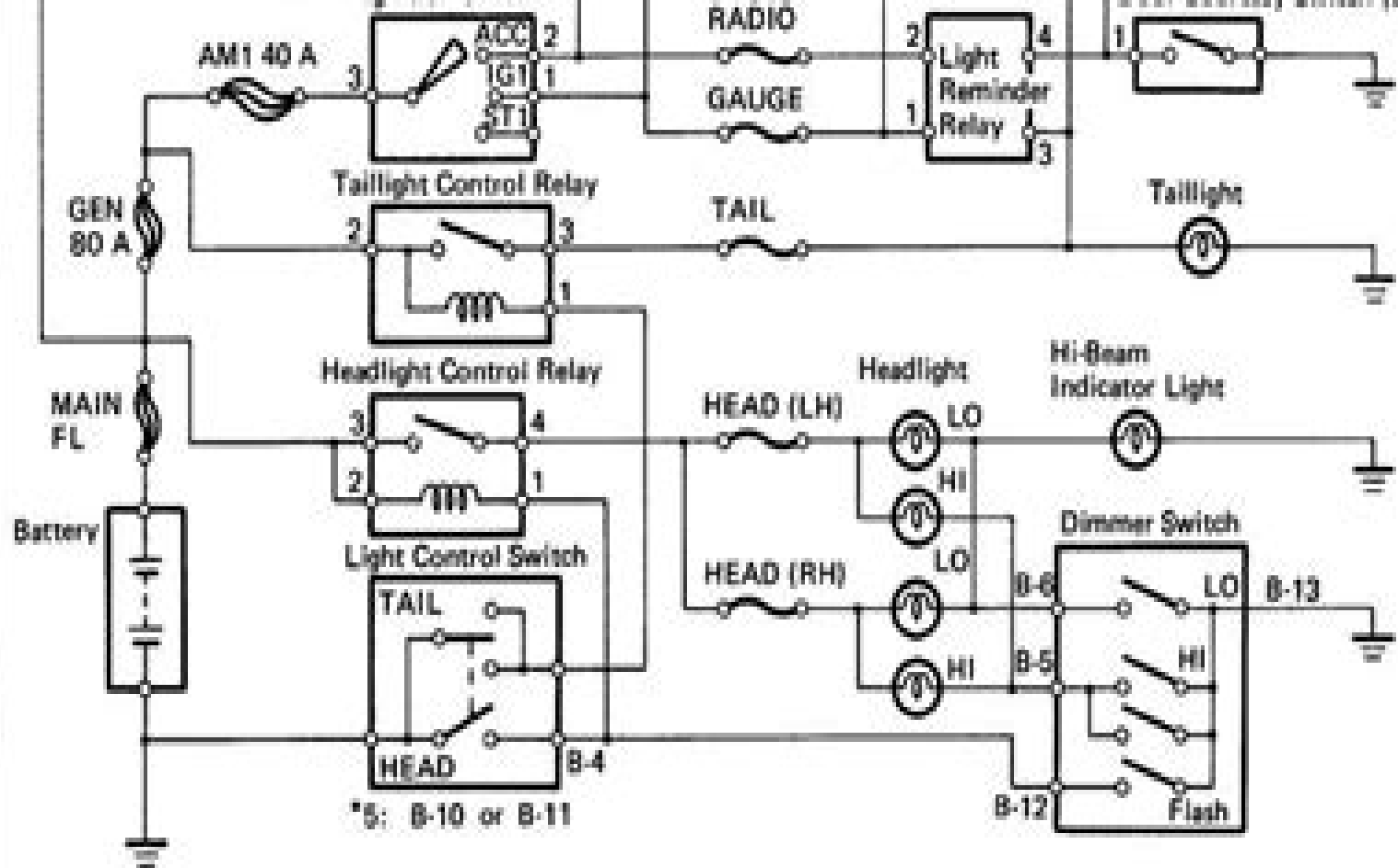
Taillight Control Relay
