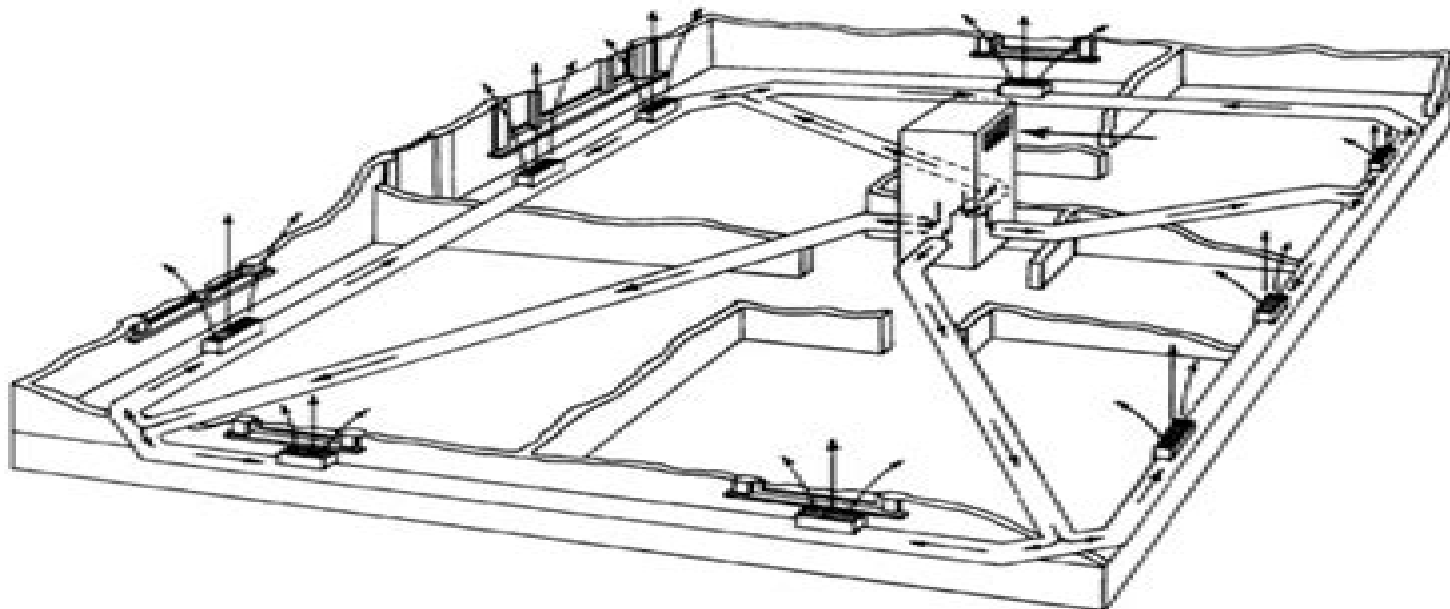
Figure 6-4. Perimeter loop delivery systems.
