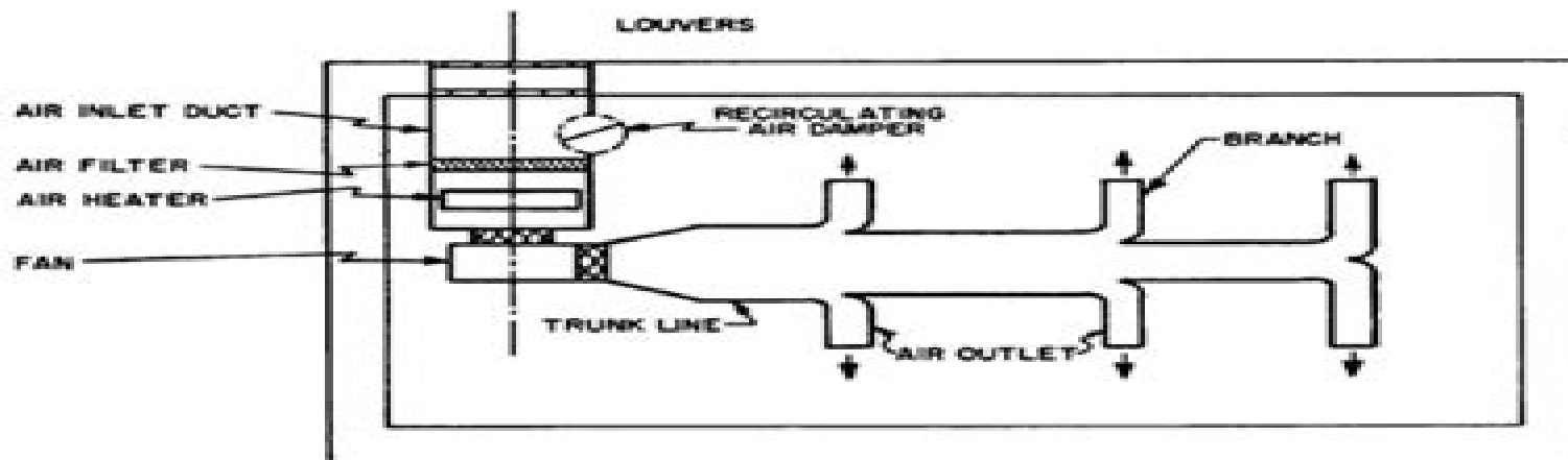
Figure 6-3. Control fan heating system.
