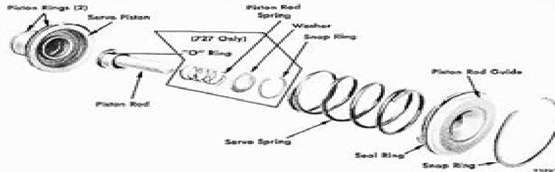
Figure 97 — Kick-Down Servos Assembly Sequence
