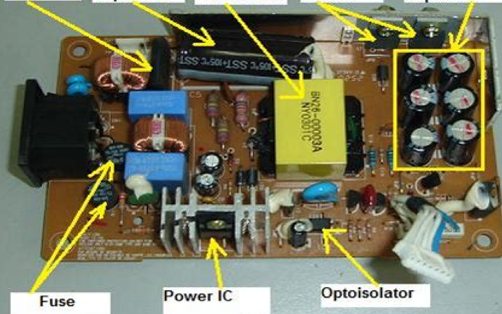
A LCD Monitor Internal Power Supply Board
