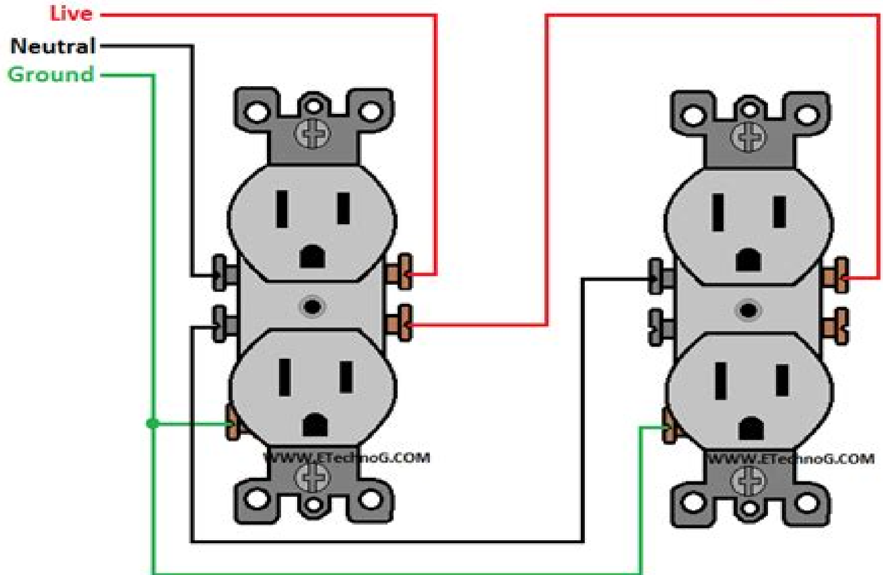
Double Outlet Wiring Diagram
