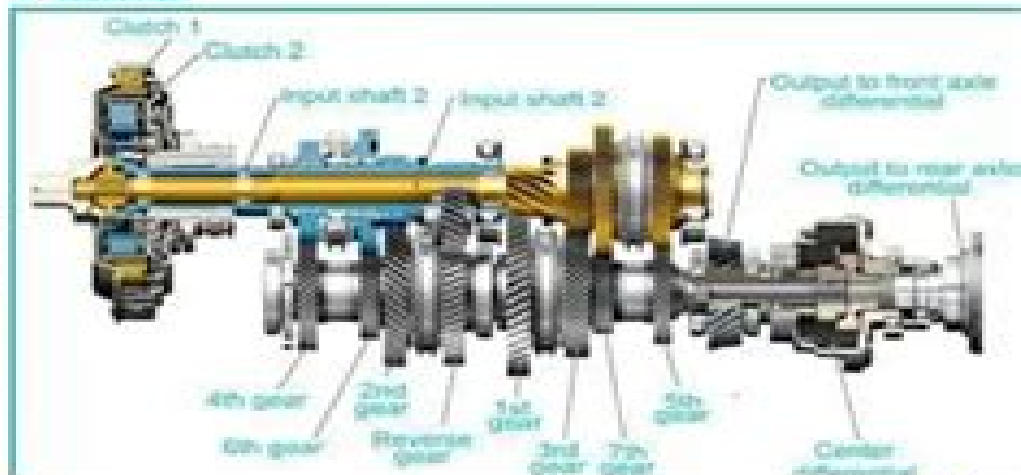
Manual Transmission System
