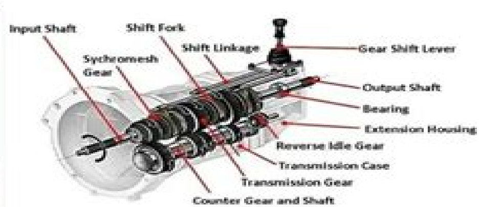
Manual Transmission System
