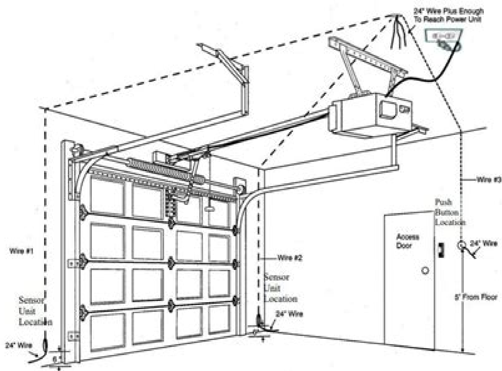
PRE WIRING FOR IR-SENSOR SYSTEM 2-Conductor Wire (white and white/black) on each side of garage door exiting ceiling
