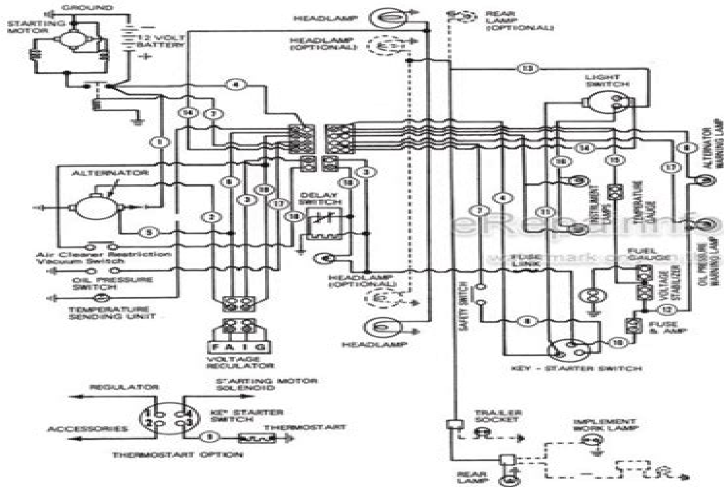
Figure 1 Electrical System Schematic
