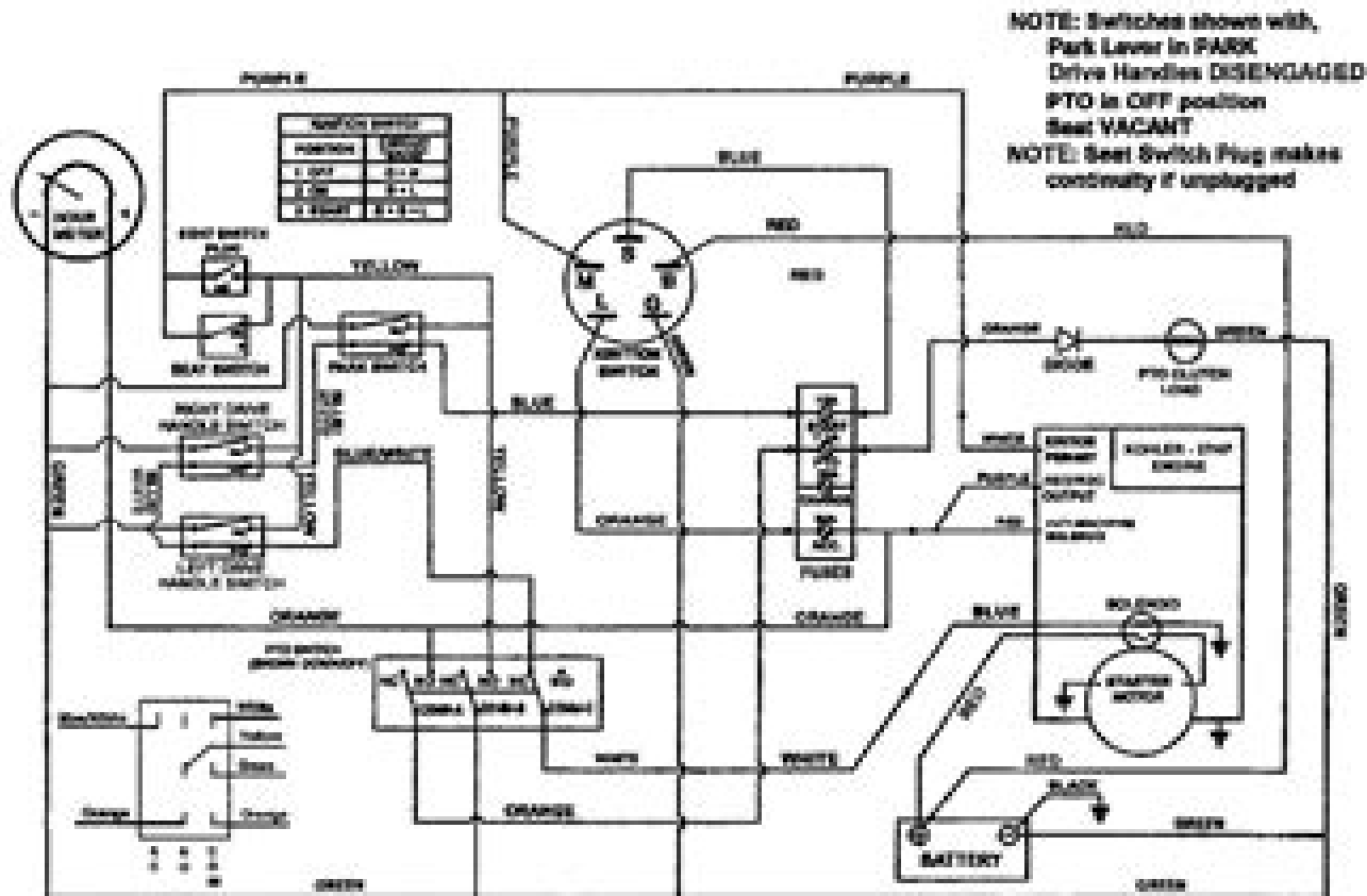
SCHEMATIC - WIRING HARNESS P.N. 29337
