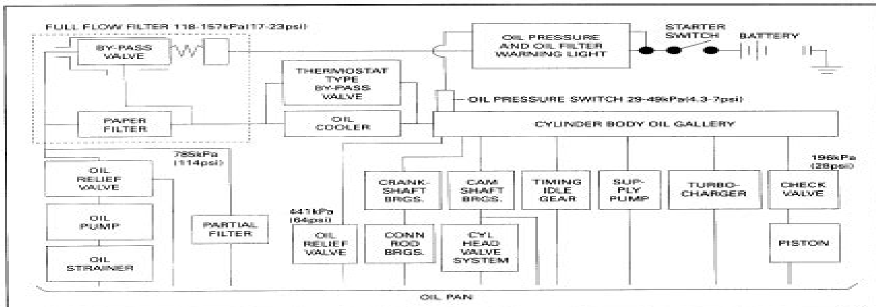
Figure 2 — Lubrication System
