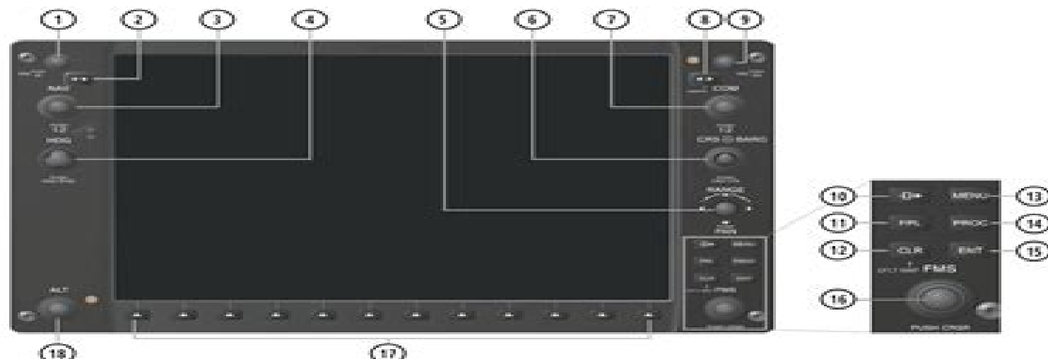
Figure 1-2 PFD/MFD Controls
