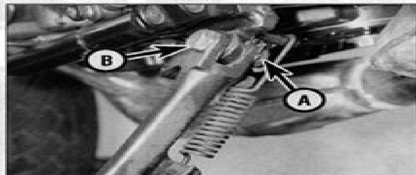
4.6 Unhook the spring, then unscrew the nut (A) and withdraw the bolt (B)
