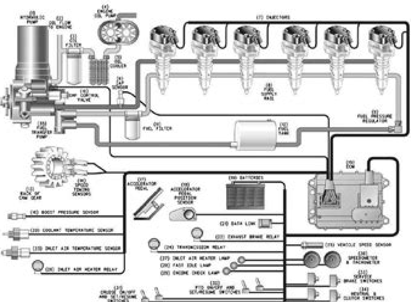
Illustration 7 Diagram of components for the engine fuel system
