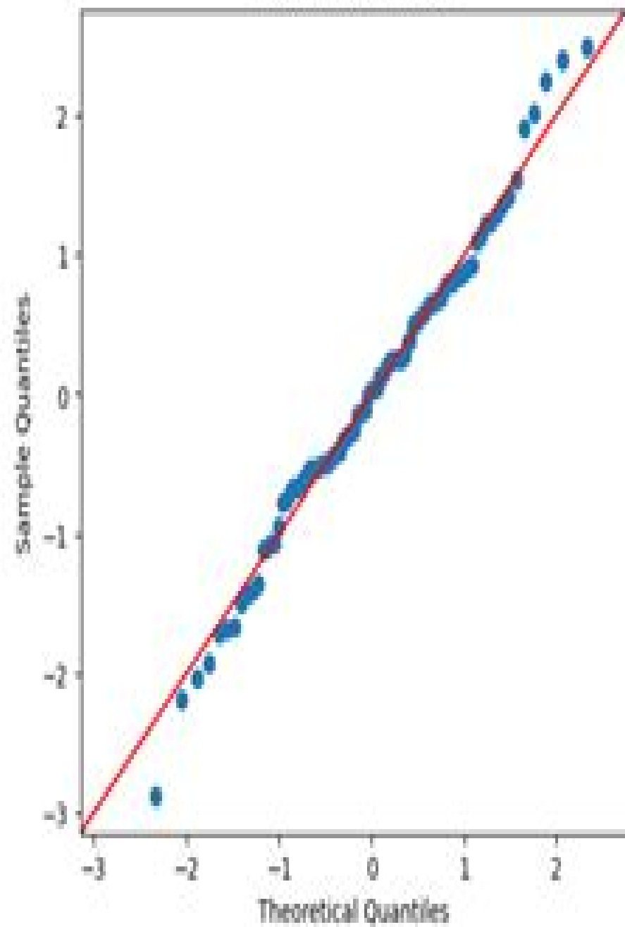
Normal Residuals
