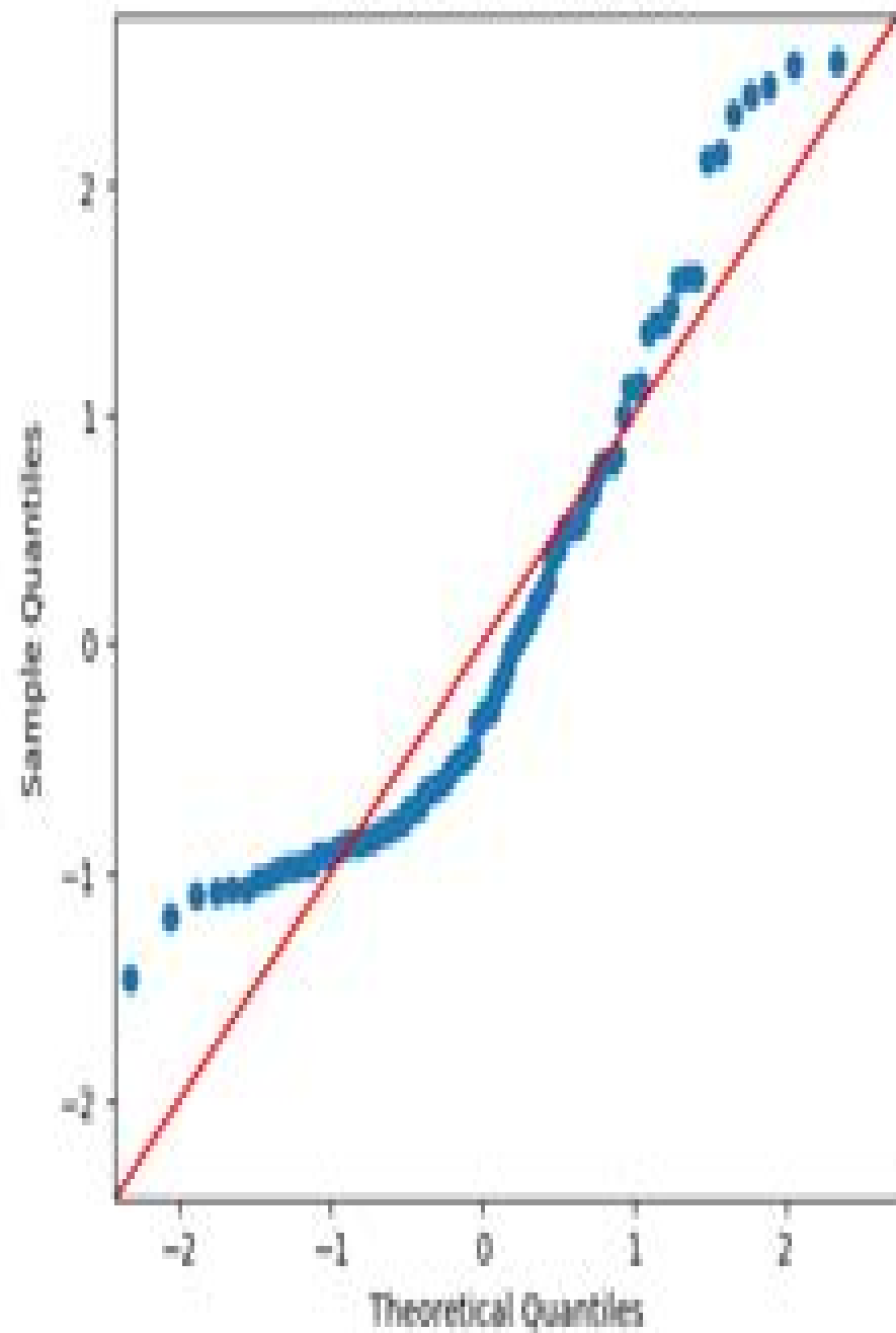
Non-Normal Residuals
