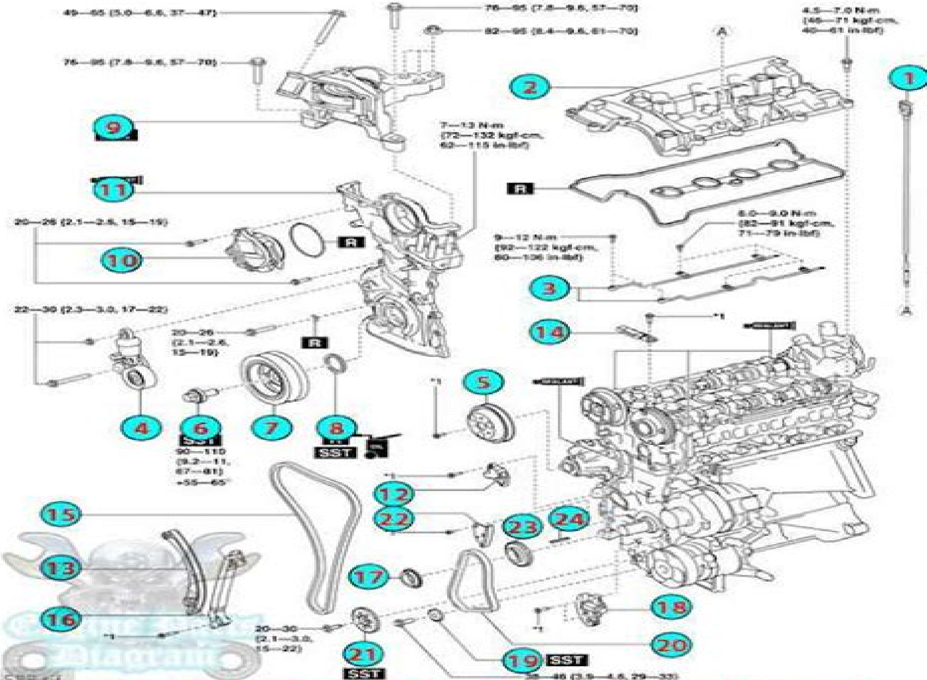
2014 Mazda 6 Timing Chain Parts Diagram (SKYACTIV-G Engine)
