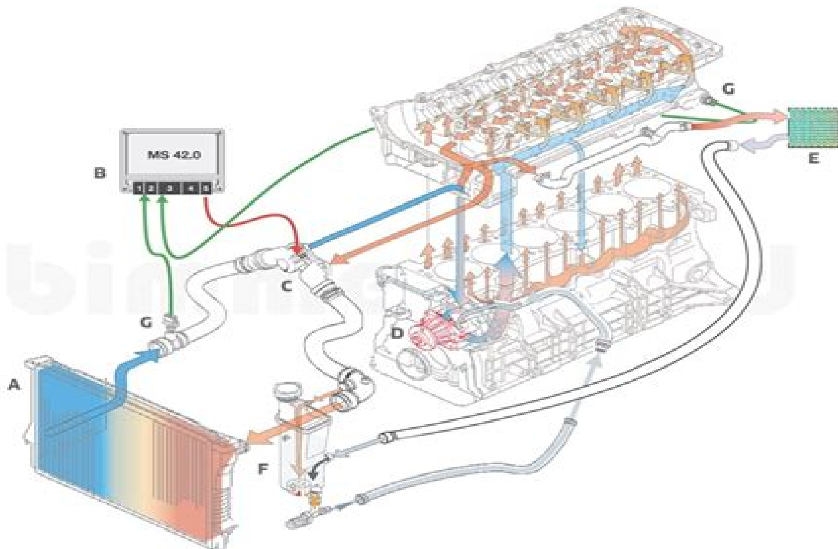
A Radiator | B DME | C Thermostat | D Water Pump | E Heater Core | F Expansion Tank | G Sensor
