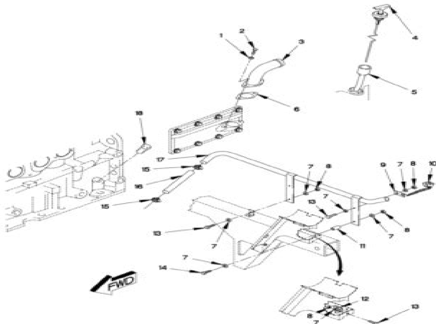
FIGURE 21. ENGINE OIL DIPSTICK AND FILLER TUBE
