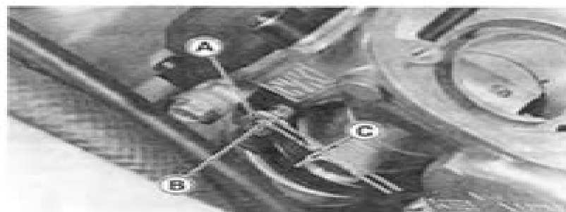
A. Starter Plunger Lever C. Play B. Starter Plunger
