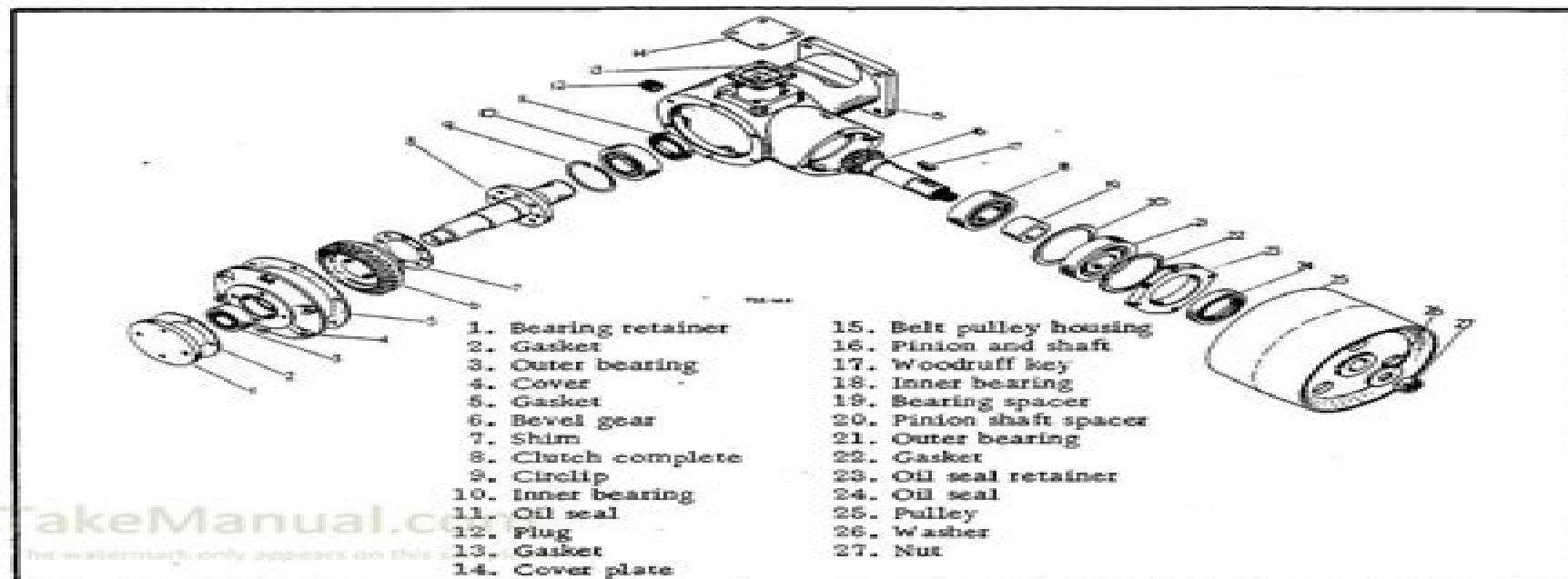
FIG. 17 EXPLODED VIEW OF THE BELT PULLEY ATTACHMENT
