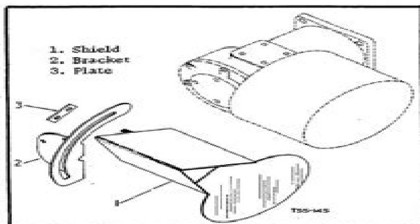
FIG. 18 BELT PULLEY AND SHIELD ATTACHMENT
