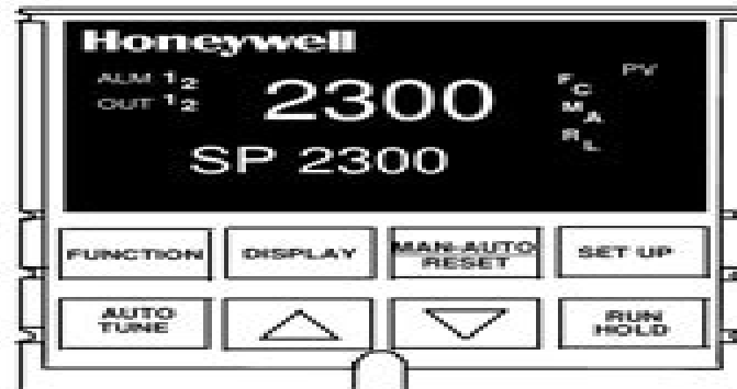
Figure 1—UDC 2300 Controller has a sealed faceplate suitable for hosedown applications
