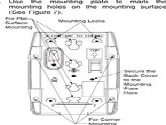
Figure 7. Mounting Plate
