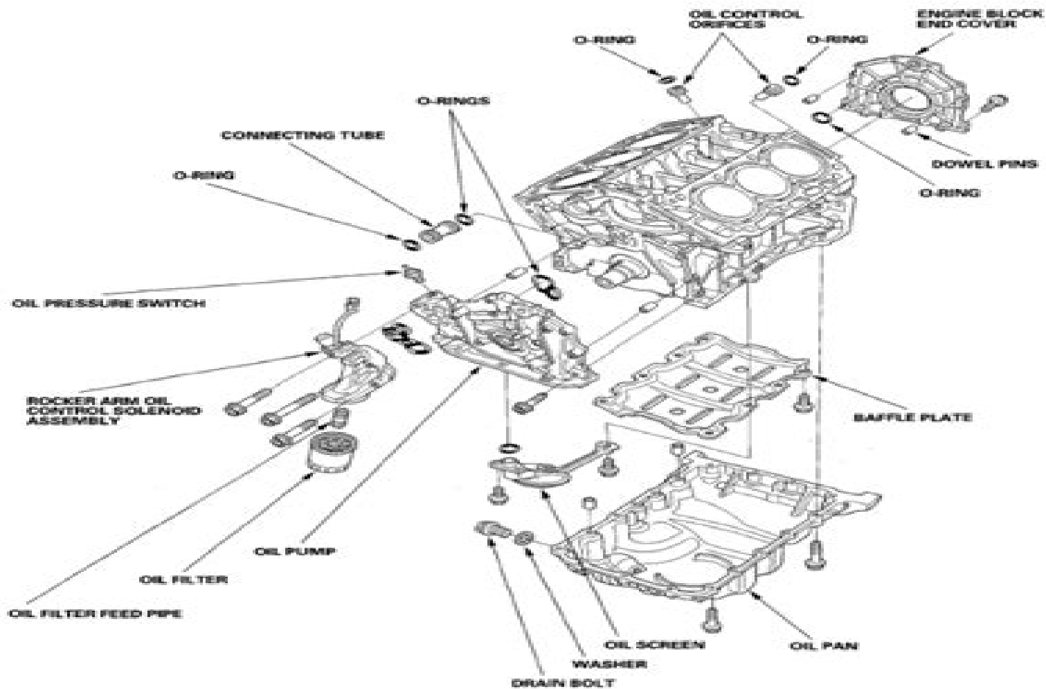
Fig. 2: Identifying Engine Lubrication Components Location (1 Of 2) Courtesy of AMERICAN HONDA MOTOR CO., INC.
