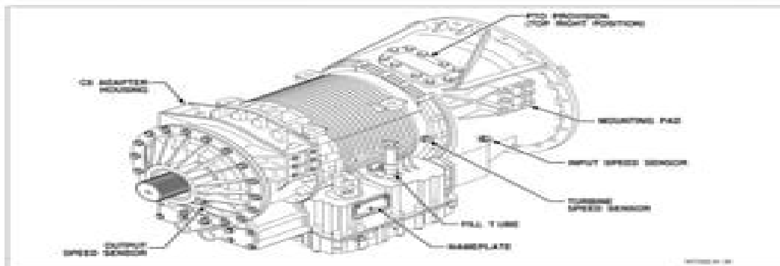
Figure 1-6. 4000 Product Family with PTO Provision (4700 and 4800 Models)—Right-Rear View
