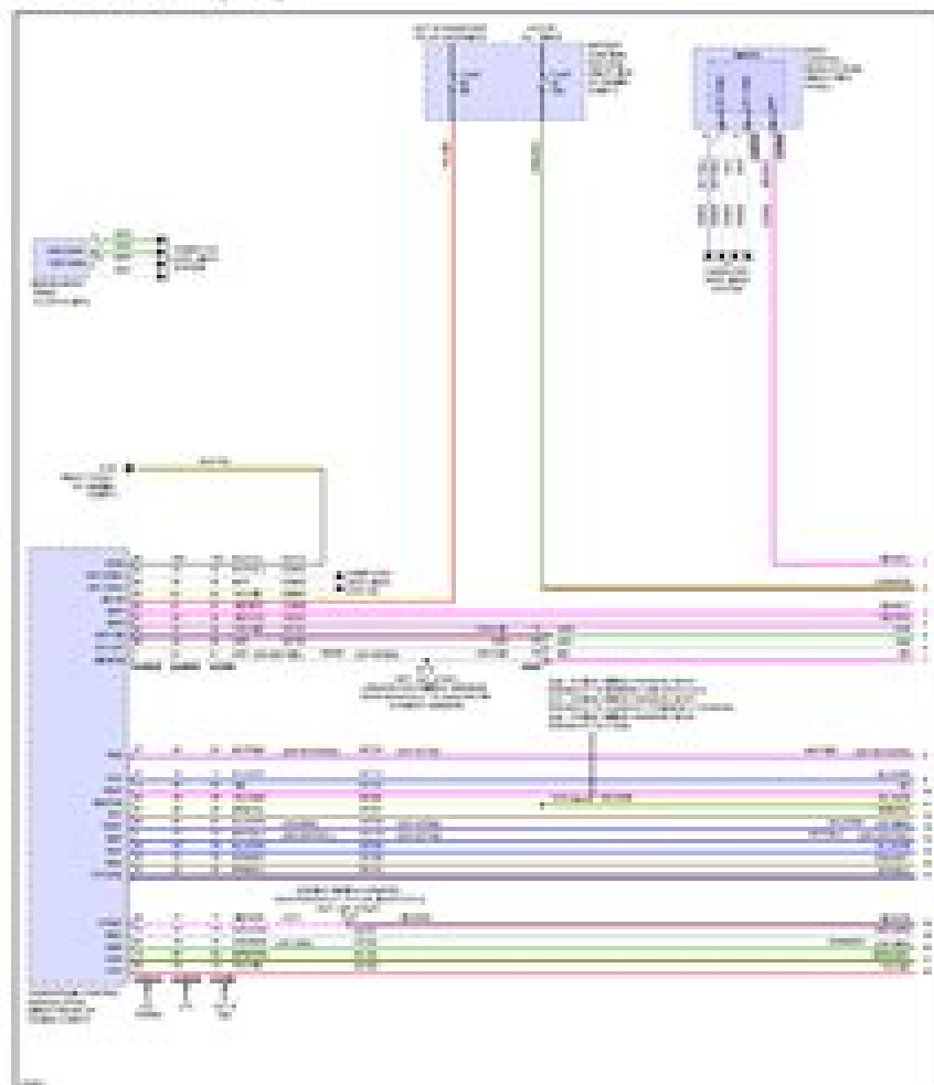
Fig 1: Transmission Circuit (1 of 2)
