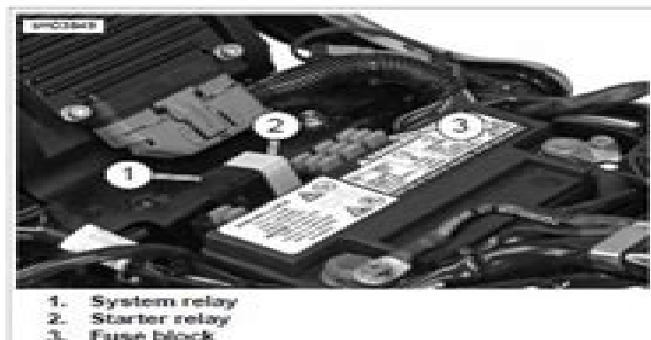
Figure 8-9. Fuse Block
