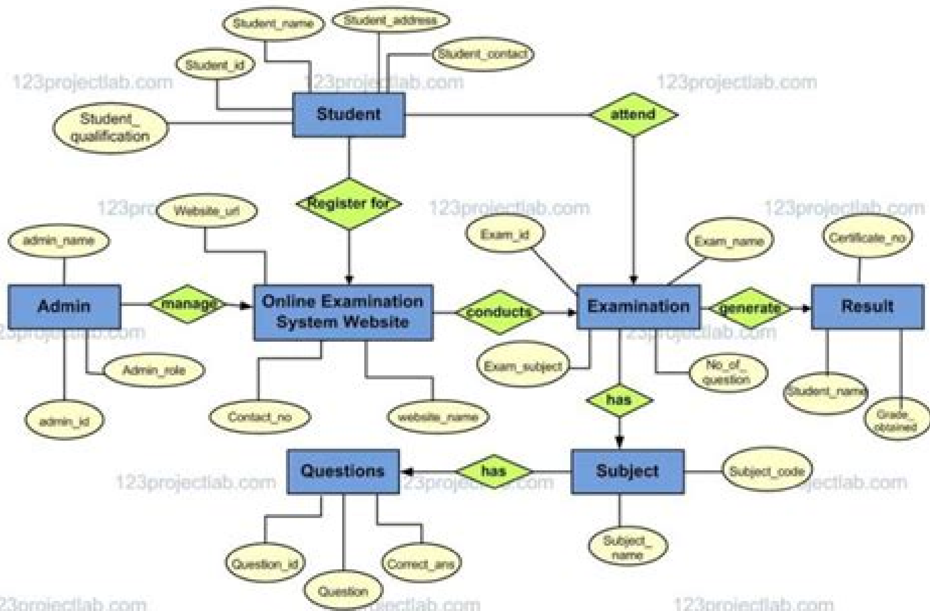
ER-Diagram for Online Examination System
