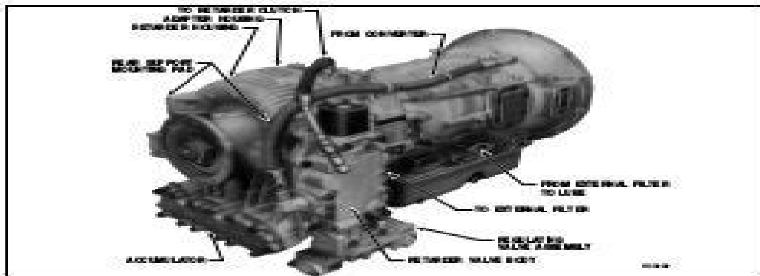
Figure 1-8. Model MTB 653 Automatic Transmission — Right-Rear View
